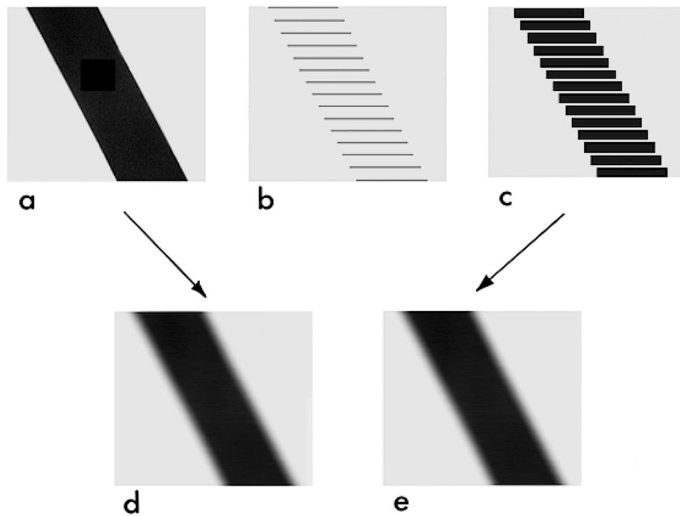
Fig. 3. a, An (x, t) plot of a bar moving to the right over time. Time proceeds downward. The vertical dimension is not shown. b, An (x, t) plot of the same bar, sampled in time. c, The sampled motion as displayed in a movie in which each frame remains on until the next one appears. d, Continuous motion after spatiotemporal blurring. e, Sampled motion after spatiotemporal blurring. The middle- and low-frequency information is almost the same for the two stimuli.
